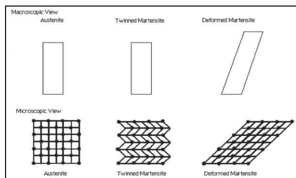
Fig 3: Microscopic and Macroscopic Views of the Two Phases of Shape Memory Alloys
