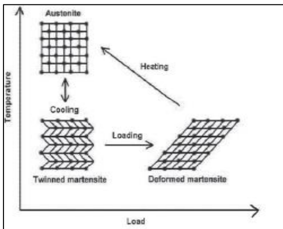
Fig 5: Microscopic Diagram of the Shape Memory Effect
